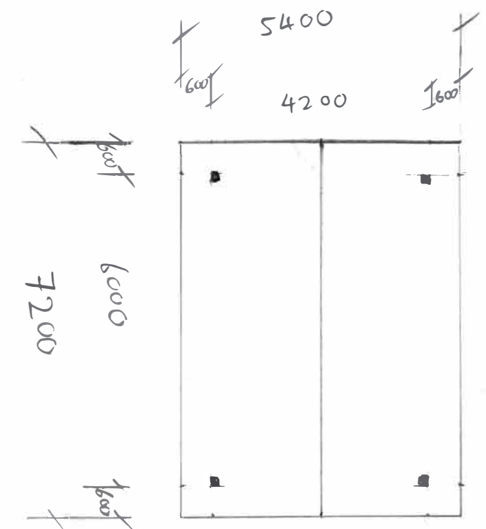
CARPORT - GABLE ROOF PLAN
